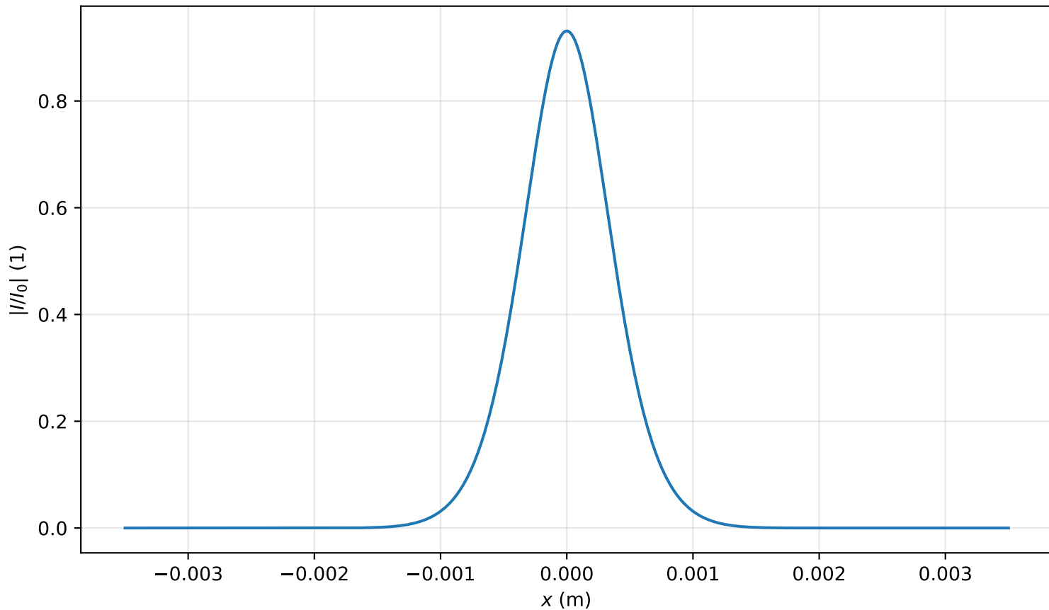
Intensity profile I(x, y = 0, z = 1.274m)/I_0 , P_{in}=0.4P_{cr} , artificial time
